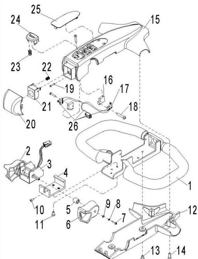
Fig.12 Handle head
